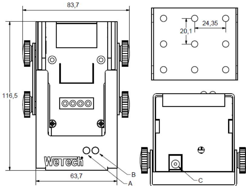
Schematic drawing WTC689
